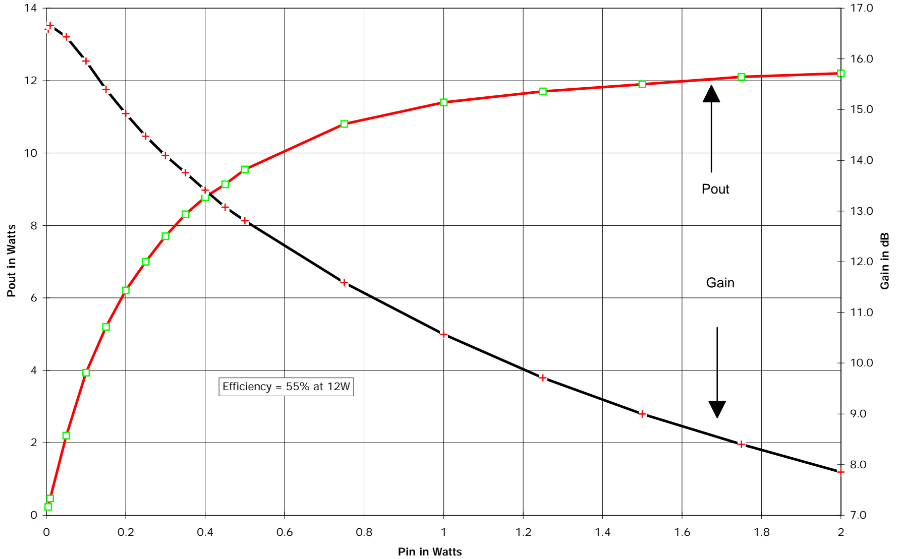
TB-142 Pin vs Pout Freq=460MHz Vds=12.5 Vdc Idq=.2A
